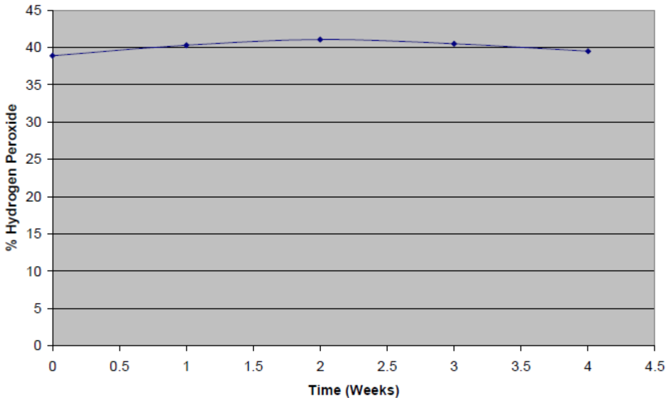
Poly-Pore 337HP Product Stability, 50 C
