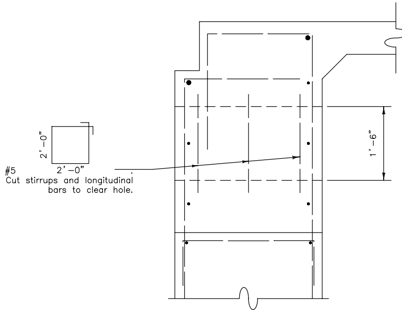
SECTION
