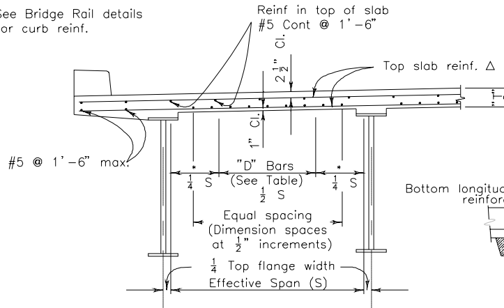
STEEL GIRDER
