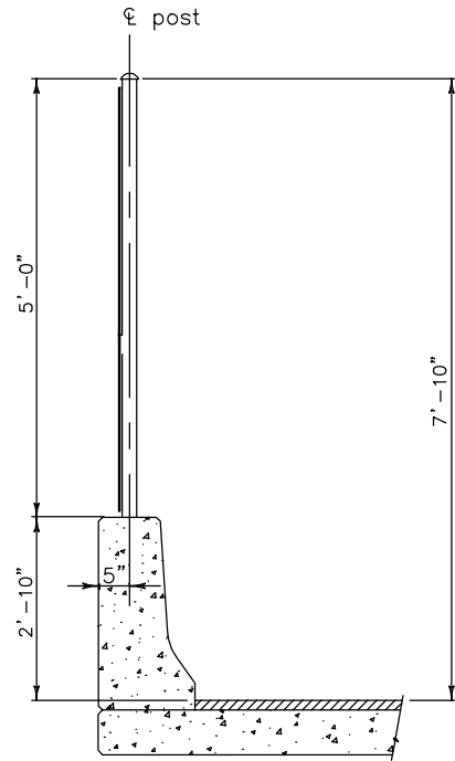
BRIDGE RAIL WITH VERTICAL FENCE
