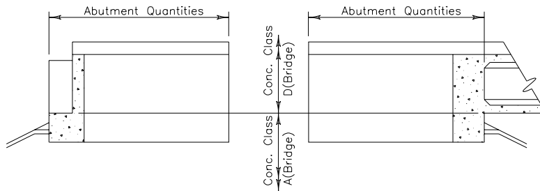
TYPICAL ABUTMENT SECTIONS & WING ELEVATIONS
