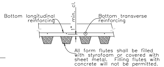
PERMANENT STEEL DECK FORM DETAIL
