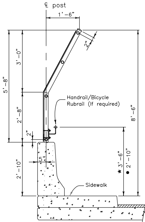
BRIDGE RAIL WITH PARTIAL ENCLOSURE
