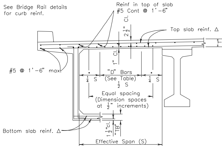
CONCRETE GIRDER
