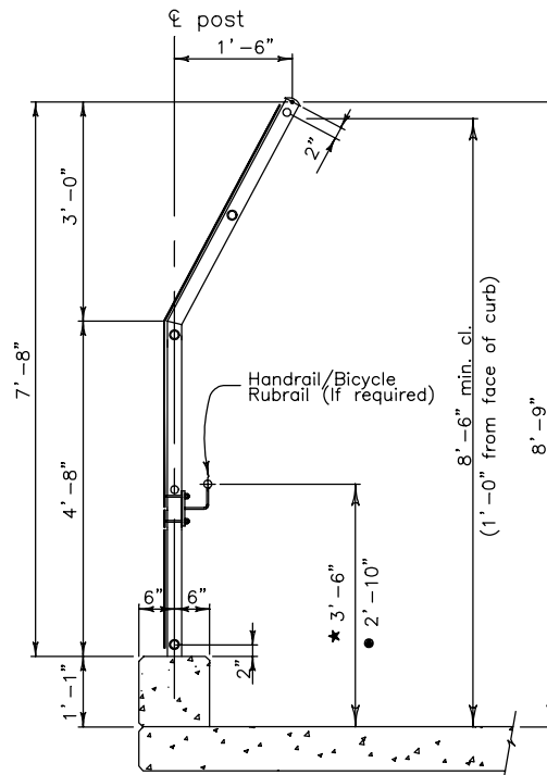
PARTIAL ENCLOSURE
