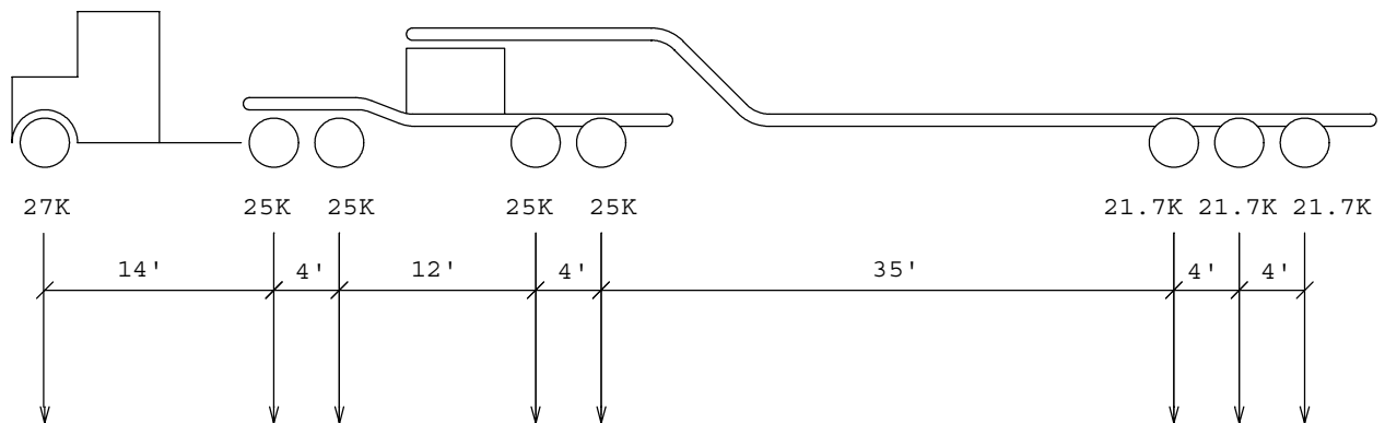
COLORADO PERMIT VEHICLE 192,000 LBS (96 Tons) on 8 Axles, 77 Feet Long
