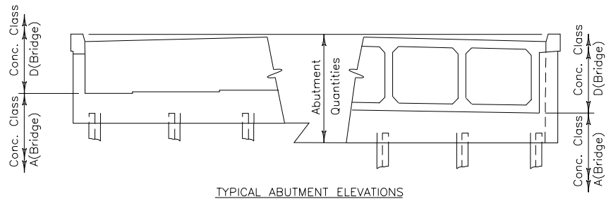
TYPICAL ABUTMENT ELEVATIONS
