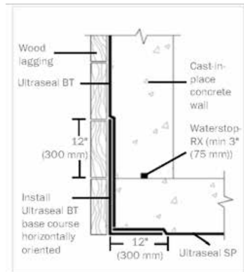
Property Line Transition Detail
