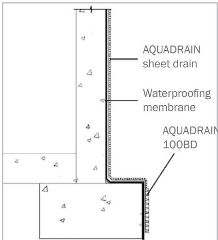
FOUNDATAION WALL
