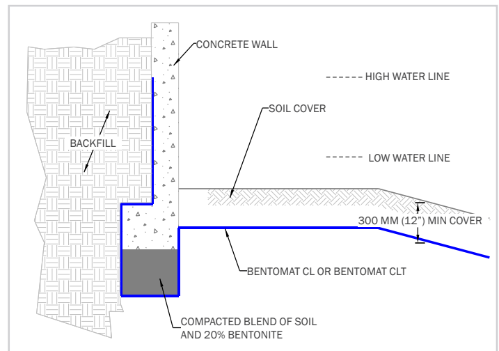
Figure 3-4. Perimeter retaining wall detail.
