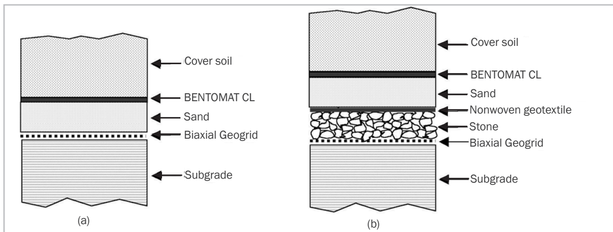
Figure 4-3. Use of geogrid and geotextile to reinforce unstable subgrade soils.
