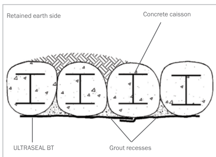
Figure 2.20 – Fill in recesses between cast caissons with grout to provide smooth surface (Plan View)
